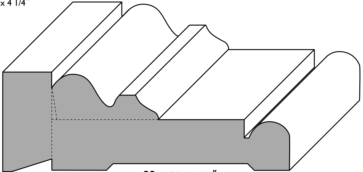
33. 1 3/4 x 4 1/4"
